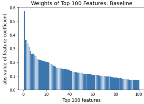
Figure 3: Weights of Top 100 Features for Johnson et al. model
