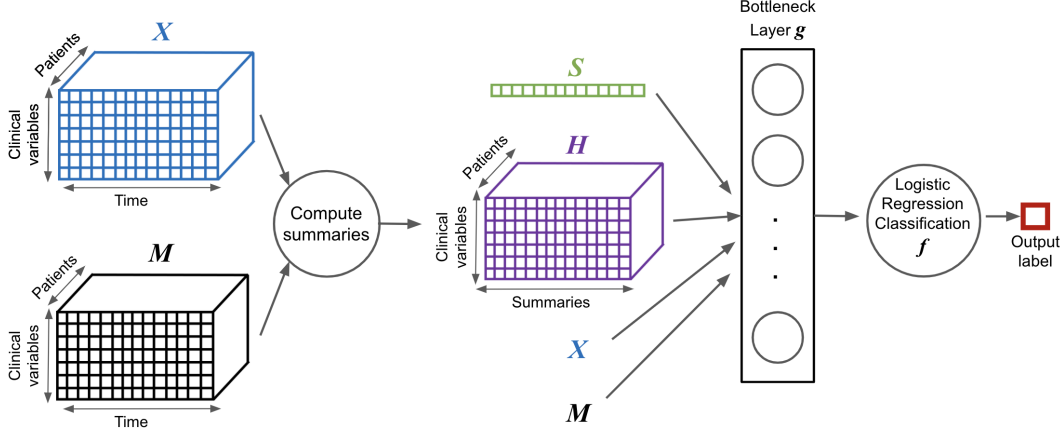
Figure 1: Our Bottleneck Model Architecture. We compute summaries H from clinical timeseries \{X, M\} , and then concatenate them with the original inputs to form Z . We then feed Z as input to function g , which outputs concepts C . Lastly, logistic regression model f uses C to output predicted probabilities for the output label y .
