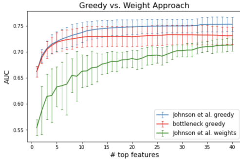
(a) Greedy vs. Weights Feature Selection Approach
