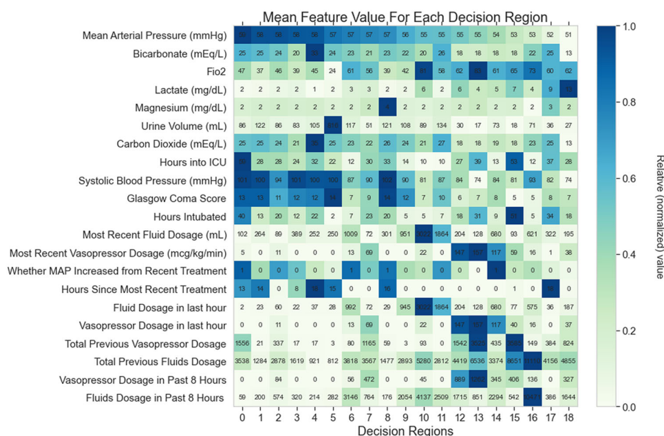
Fig. 3 The feature means for points in each decision region. Means are sorted by descending order of Mean Arterial Pressure (MAP) value.
