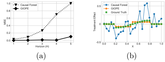
Figure 7: Toy MDP: (a) Mean squared error of treatment effect prediction for our method and causal forest(CF). (b) True and predicted treatment effect for different values of x for our method and causal forest.
