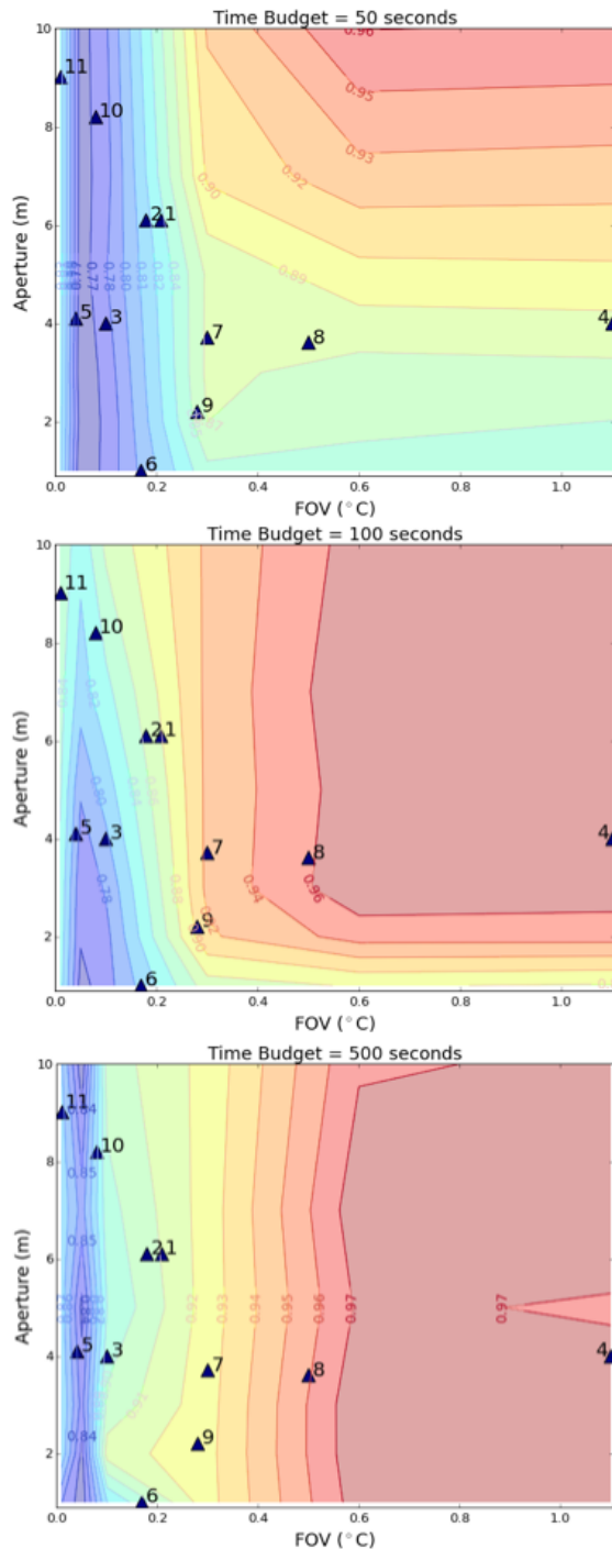
Figure 4: Contour plot of accuracy as a function of FOV and aperture with different time cost budgets.
