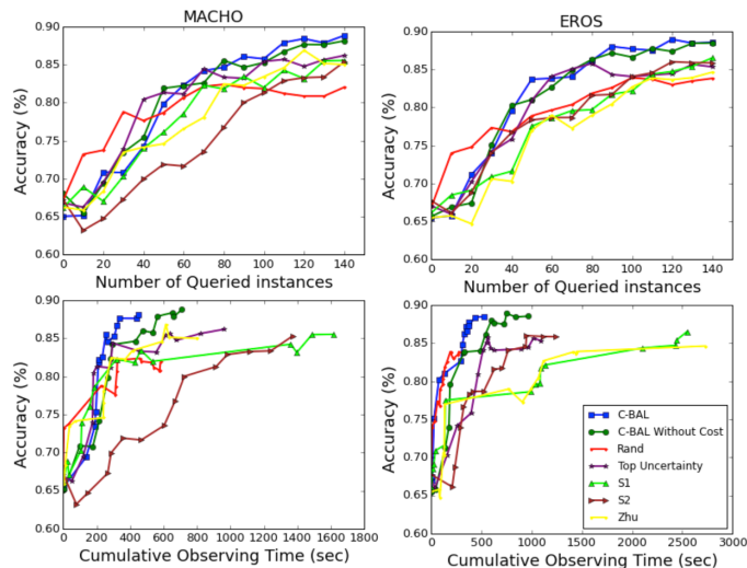
Figure 1: Comparative performance of different active learning methods on MACHO and EROS data sets.
