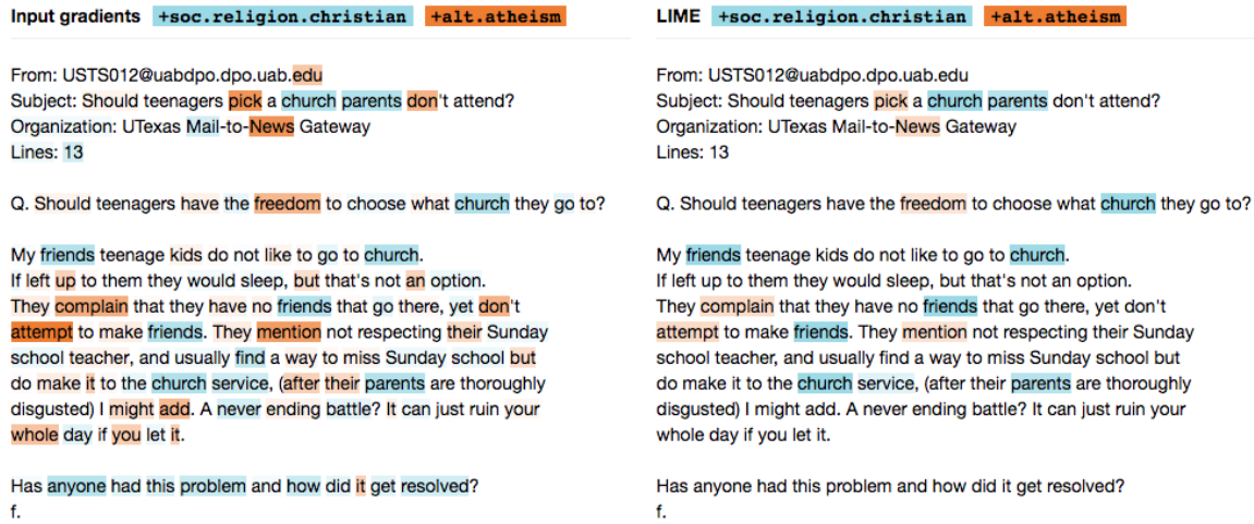
Figure 5: Words identified by LIME vs. gradients on an example from the atheism vs. Christianity subset of 20 Newsgroups. More examples are available at https://github.com/dtak/rrr . Words are blue if they support soc.religion.christian and orange if they support alt.atheism, with opacity equal to the ratio of the magnitude of the word’s weight to the largest magnitude weight. LIME generates sparser explanations but the weights and signs of terms identified by both methods match closely. Note that both methods reveal some aspects of the model that are intuitive (“church” and “service” are associated with Christianity), some aspects that are not (“13” is associated with Christianity, “edu” with atheism), and some that are debatable (“freedom” is associated with atheism, “friends” with Christianity).
