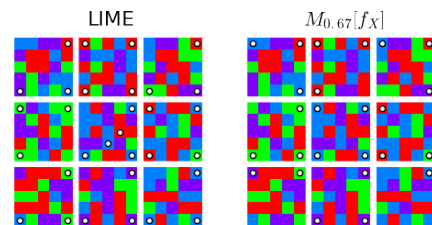
Figure 2: Gradient vs. LIME explanations of nine perceptron predictions on the Toy Color dataset. For gradients, we plot dots above pixels identified by M_{0.67} [f_X] (the top 33% largest-magnitude input gradients), and for LIME, we select the top 6 features (up to 3 can reside in the same RGB pixel). Both methods suggest that the model learns the corner rule.
